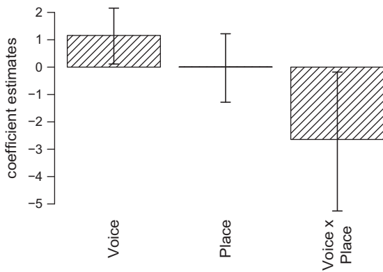
Fig. 2. Markov Chain Monte Carlo (MCMC) estimates of the effects of changes in Place and Voice on VOT deviance (ms) in the EPG analysis of tongue-twisters from Experiment 1. Error bars show 95% confidence intervals.
