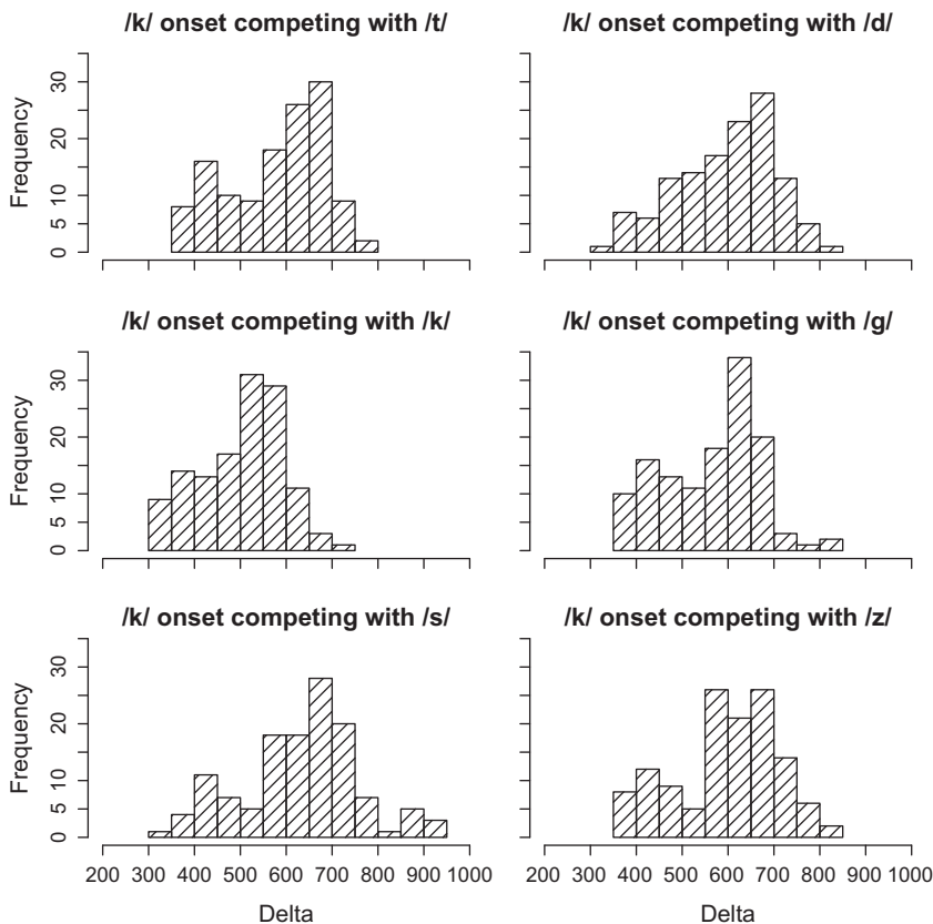
Fig. 12. Distributions of Delta for cases in which participants attempted to produce /k/ onsets (8 participants, 768 observations).
