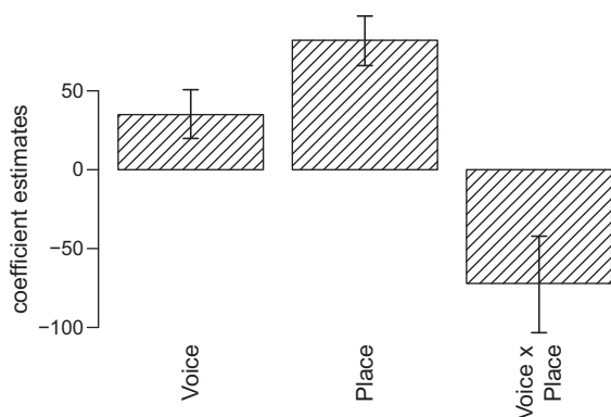
Fig. 7. Markov Chain Monte Carlo (MCMC) estimates of the effects of changes in Place and Voice on articulatory variation ( Delta ) in the EPG analysis of tongue-twisters from Experiment 2 (subset excluding /s/ and /z/). Error bars show 95% confidence intervals.
