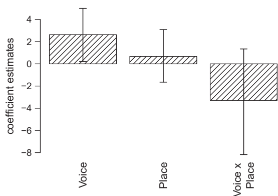
Fig. 6. Markov Chain Monte Carlo (MCMC) estimates of the effects of changes in Place and Voice on VOT deviance (ms) in the EPG analysis of tongue-twisters from Experiment 2 (subset excluding /s/ and /z/). Error bars show 95% confidence intervals.
