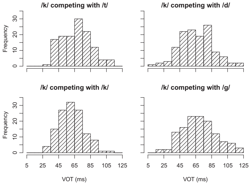
Fig. 10. Distributions of VOTs for cases in which participants attempted to produce /k/ onsets (8 participants, 509 observations).
