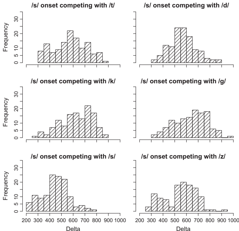
Fig. 13. Distributions of Delta for cases in which participants attempted to produce /s/ onsets (8 participants, 752 observations).
