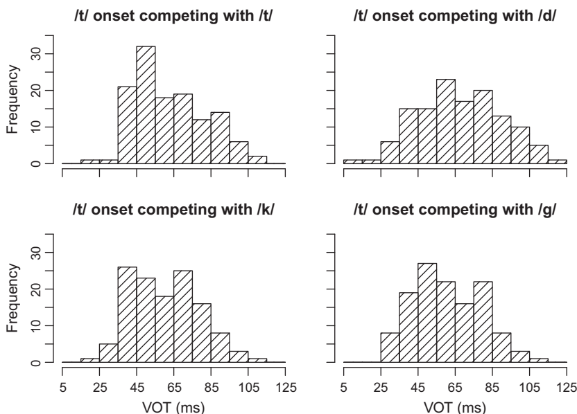
Fig. 9. Distributions of VOTs for cases in which participants attempted to produce /t/ onsets (8 participants, 505 observations).
