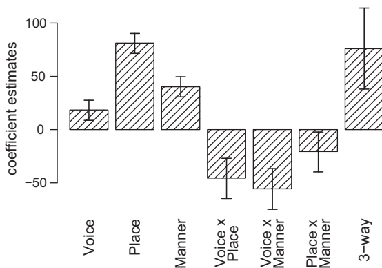
Fig. 8. Markov Chain Monte Carlo (MCMC) estimates of the effects of changes in Place, Voice and Manner on articulatory variation ( Delta ) in the EPG analysis of tongue-twisters from Experiment 2 (all data). Error bars show 95% confidence intervals.
