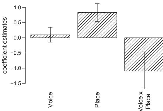
Fig. 3. Markov Chain Monte Carlo (MCMC) estimates of the effects of changes in Place and Voice on articulatory variation ( Delta ) in the EPG analysis of tongue-twisters from Experiment 1. Error bars show 95% confidence intervals.
