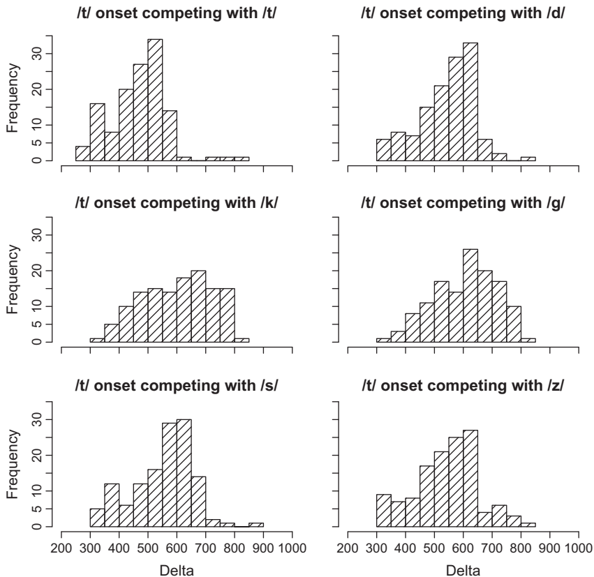
Fig. 11. Distributions of Delta for cases in which participants attempted to produce /t/ onsets (8 participants, 767 observations).
