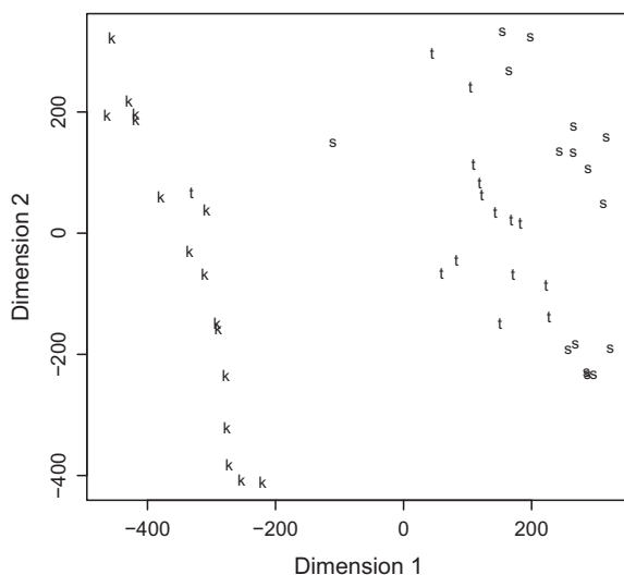
Fig. 5. Comparison of 16 /k/, 16 /t/, and 16 /s/ articulations recorded with ultrasound. Delta was calculated for each articulation relative to every other articulation. The dimensionality of the resulting deviance scores was reduced using multidimensional scaling.
